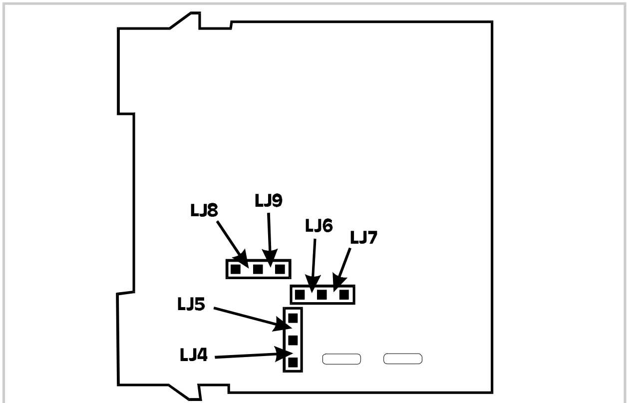
Figure 2-7 PSU PCB - \frac{1}{4} -DIN & \frac{1}{8} -DIN Controllers
