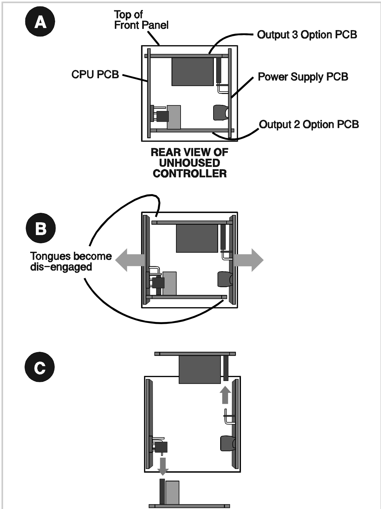
Figure 2-2 Removing the Output 2/Output 3 Option PCBs
