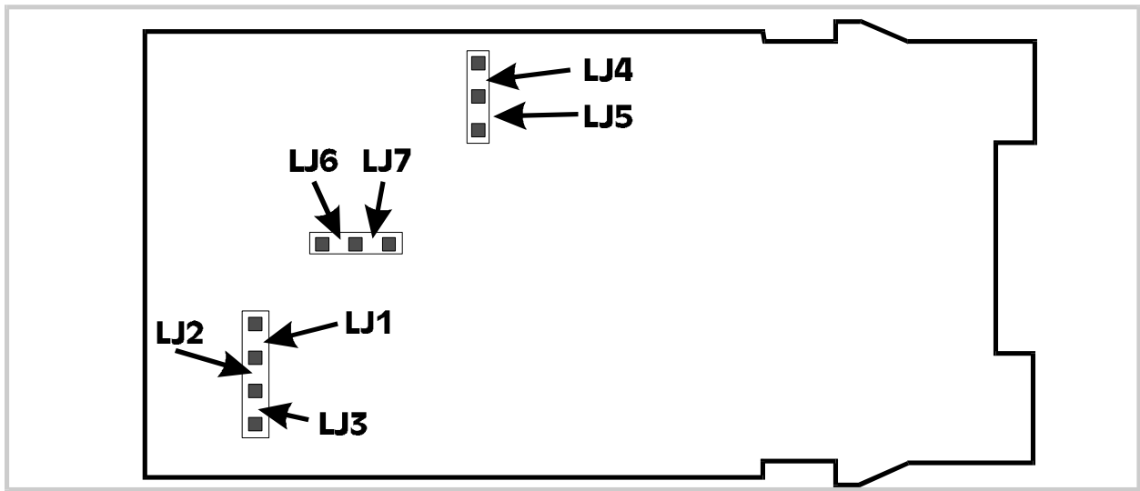
Figure 2-4 CPU PCB (Relay/SSR Drive/Solid State Output 1) - \frac{1}{16} -DIN Controllers
