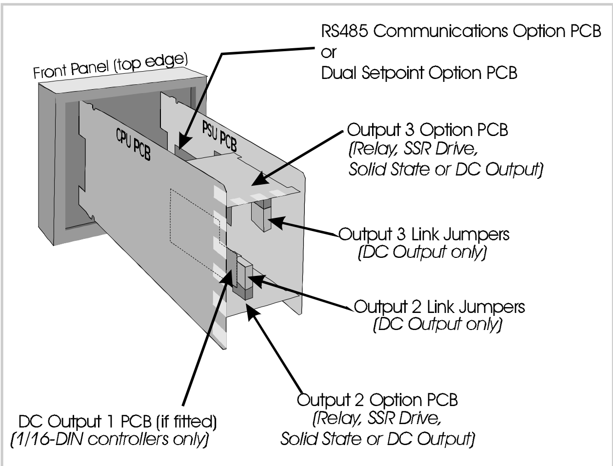
Figure 2-1 PCB Positions
