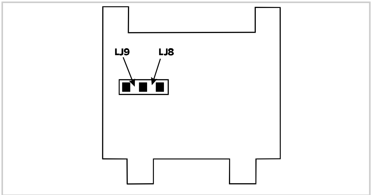
Figure 2-8 DC Output Option PCB PCB (Output 2/Output 3)
