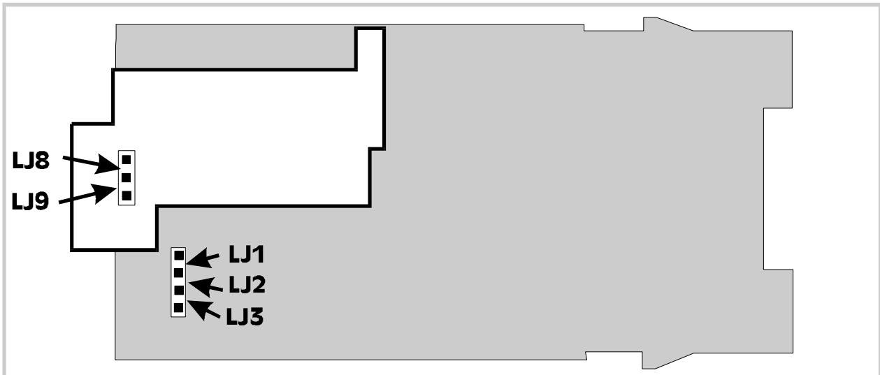
Figure 2-5 CPU PCB (DC Output 1) - \frac{1}{16} -DIN Controllers
